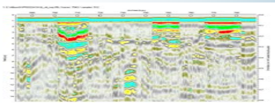
Radar profile showing amplitude variation from full depth asphalt patch repairs indicative of delamination of asphalt layers.
